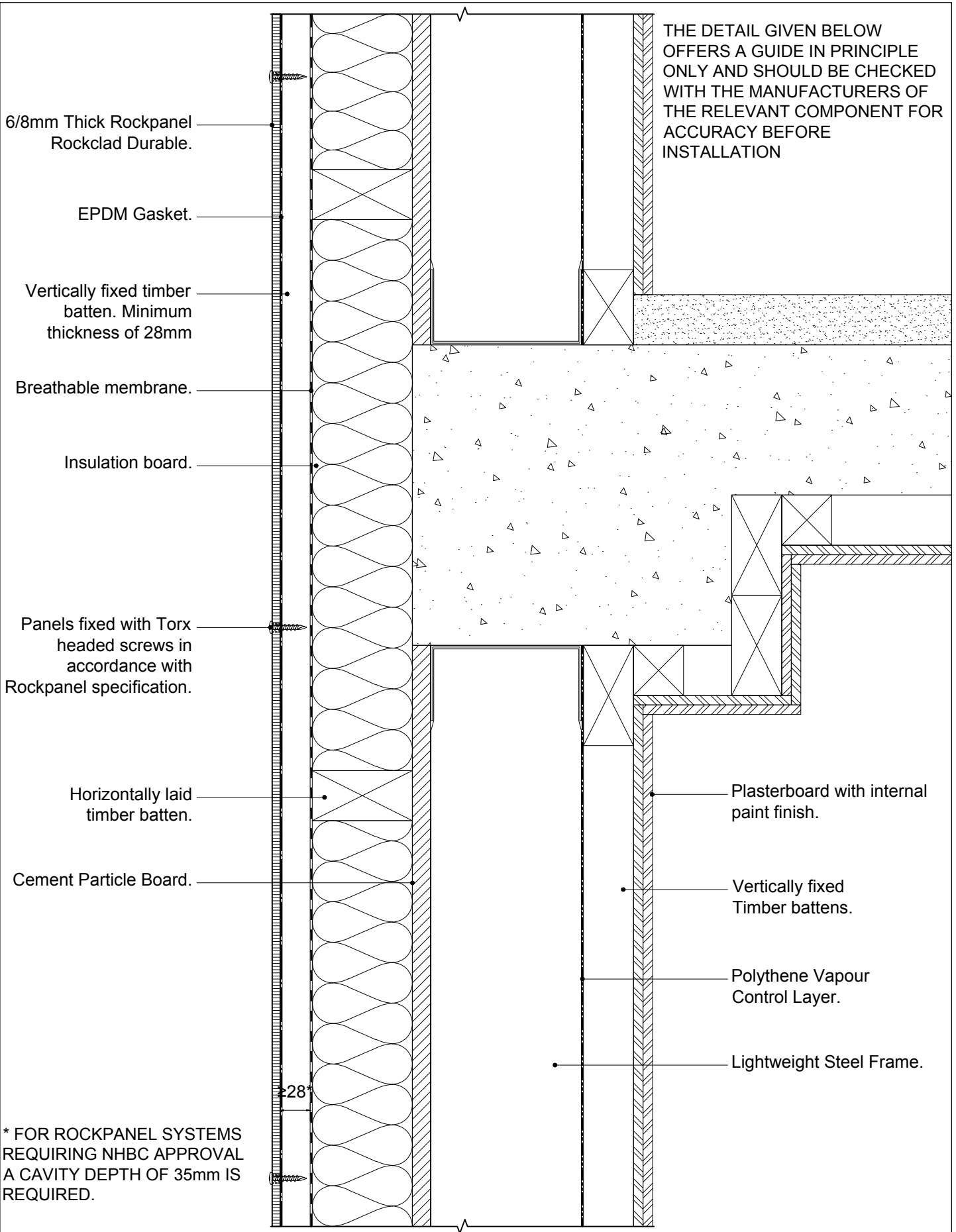
DETAIL 3 - ROCKCLAD DURABLE VERTICAL SECTION TIMBER SUBSTRUCTURE TO STRUCTURAL CONCRETE WITH LIGHT STEEL FRAME.
