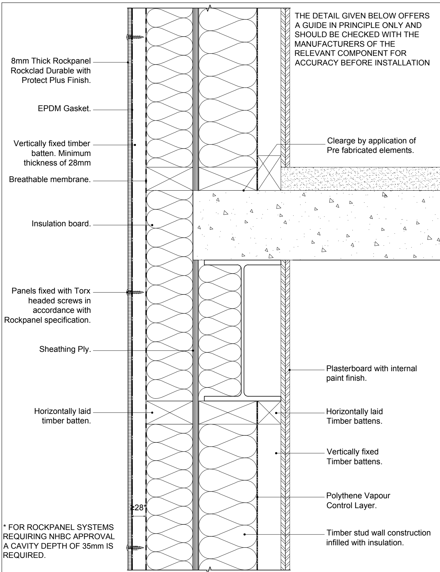
DETAIL 15 - ROCKCLAD DURABLE WITH PROTECT PLUS FINISH VERTICAL SECTION TIMBER SUBSTRUCTURE TO STRUCTURAL STEEL WITH TIMBER STUD FRAME.
